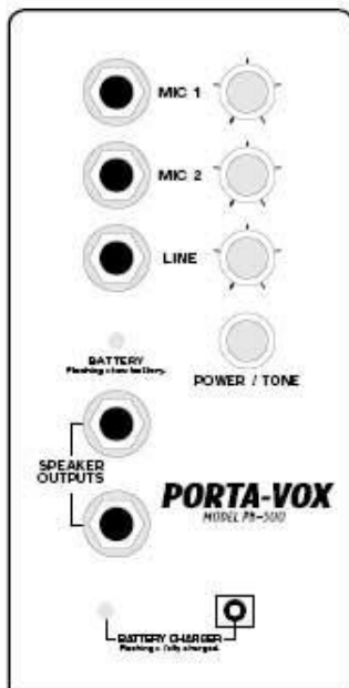
Diagram of Porta-Vox control panel.
