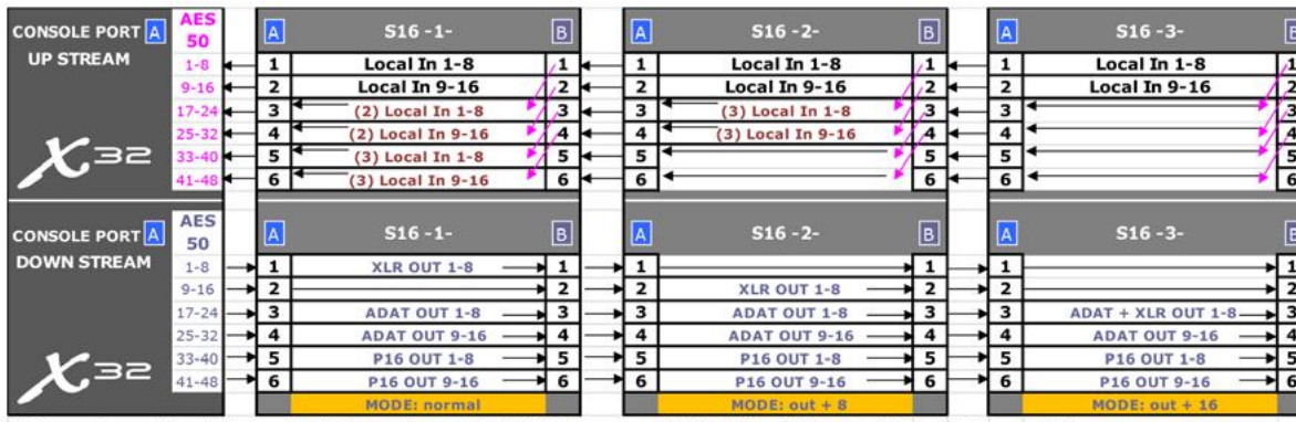
FOH console supplies clock synchronization and controls the S16 preamps exclusively (local HA control is blocked by console)
