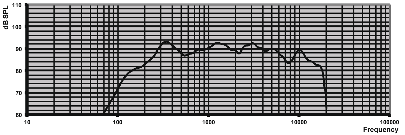
Fig. 10: Frequency response
