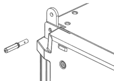
Fig. 4. Use tool to remove pin
