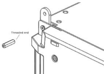
Fig. 3. Remove pin using threaded end of tool
