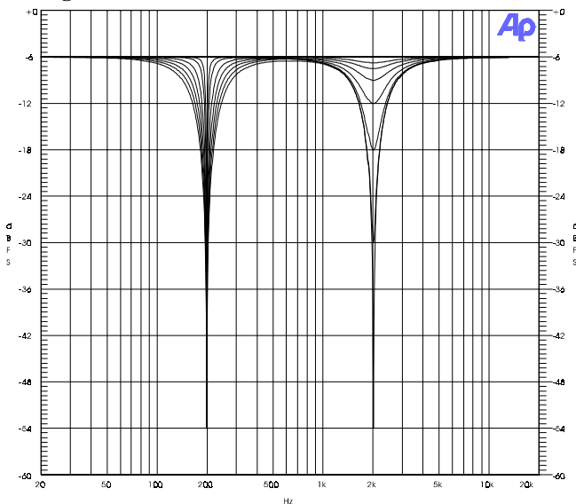
Figure 5— Notch Filter
