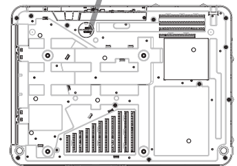
Battery Cover
