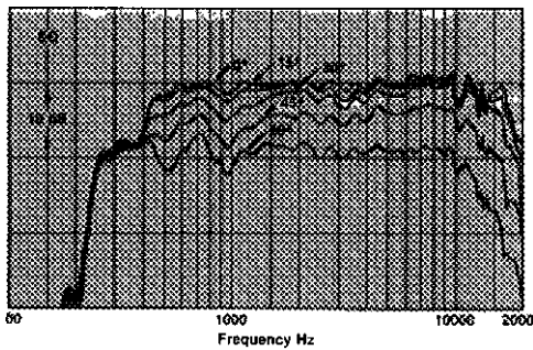
Horizontal off-axis response. Horizontal off-axis response taken at 15 degree intervals out to 60° off axis. Both normalized (equalized flat on axis) and unnormalized responses are shown.
