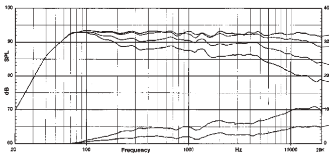
LSR32 Response Curves
