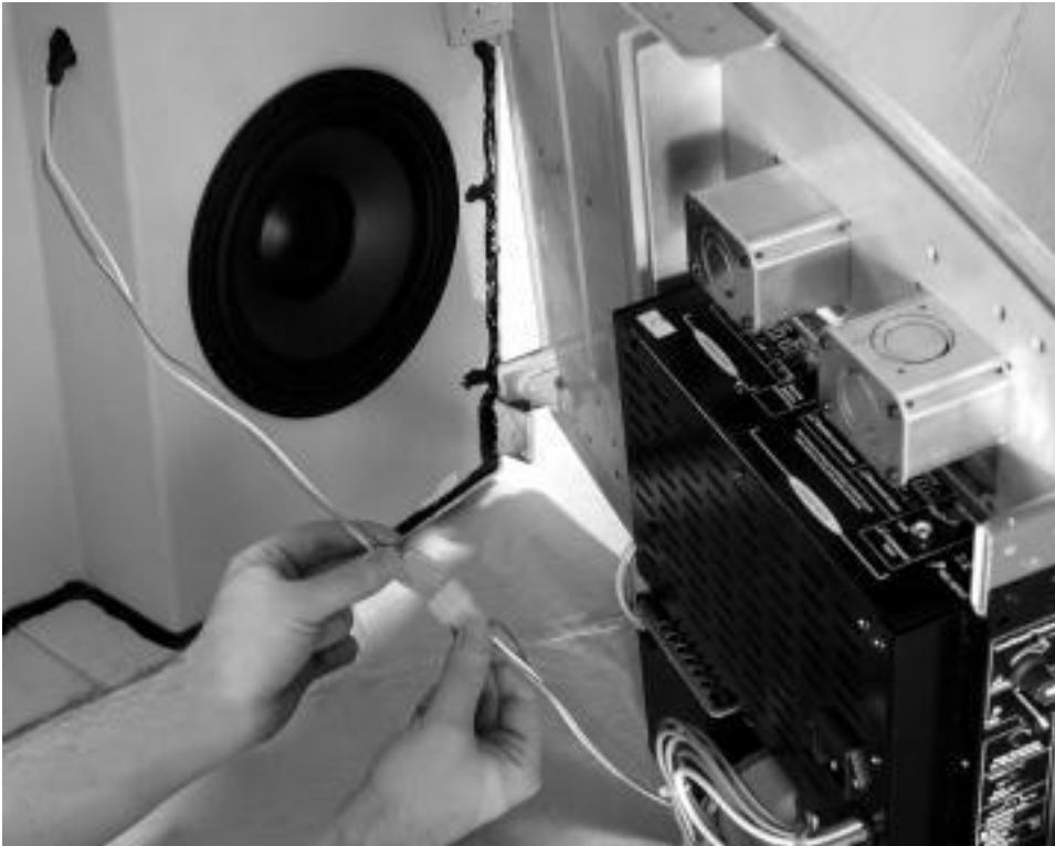
Figure 8: Connecting the Subwoofer Driver
