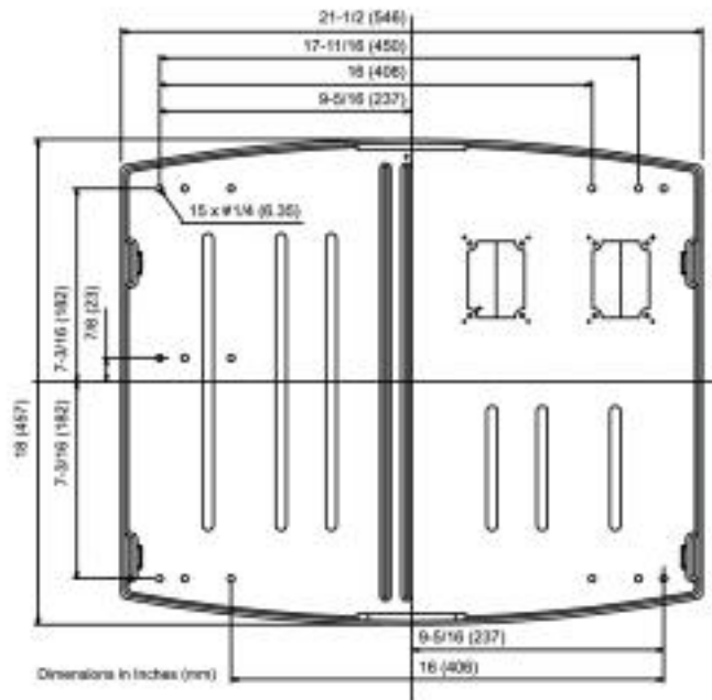
Figure 7 – Wall Baffle Mounting Holes
