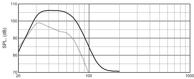
Frequency Response (solid line) of a single VT4880ADP with 80 Hz Subwoofer Filter Enabled (dashed line). Additional presets available for DP-AN, DP-CN models.
