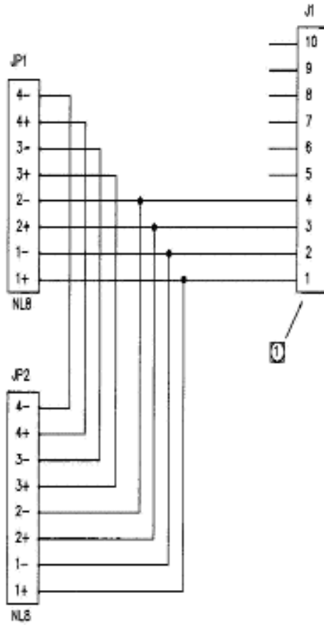
Connector Assembly 350991-001
