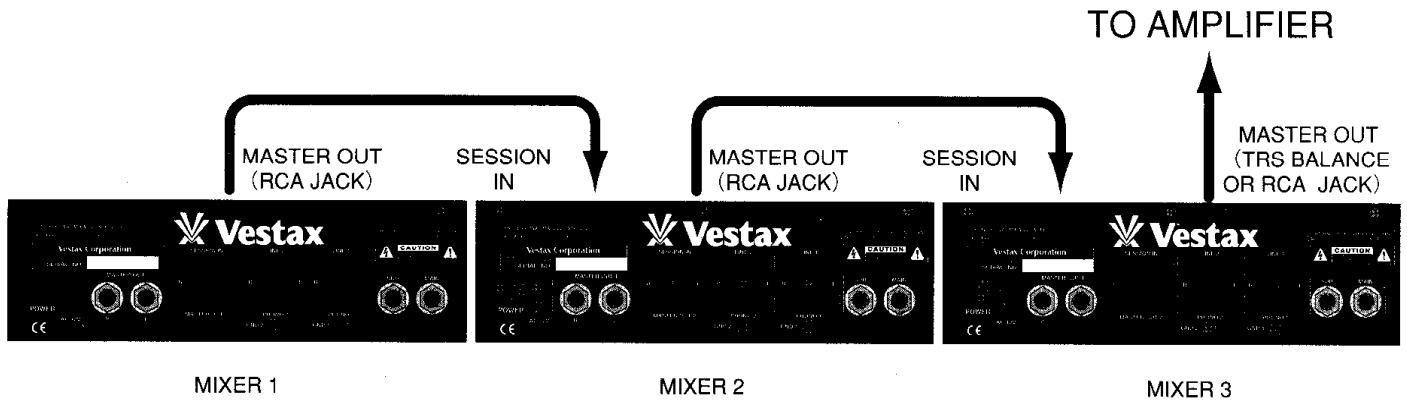
fig.4 CHAIN CONNECTION < EXAMPLE >
