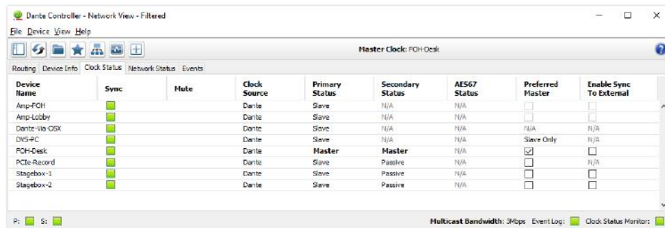
Figure 5 - Dante Controller 'Clock Status' tab
