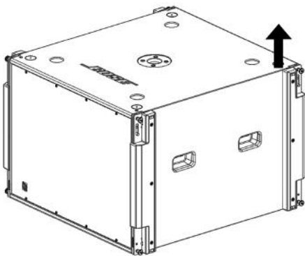
Threaded Inserts: WLL = 200 lbs (90 kg) (4x top and 4x bottom) Note: Use with custom installation rigging
