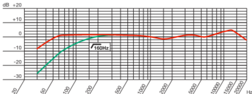
Frequency Response C214
