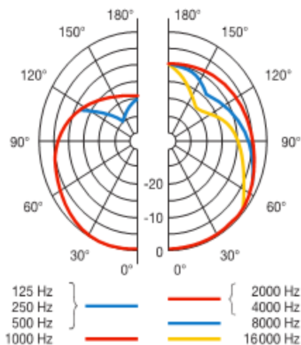
Polar Diagram C214
