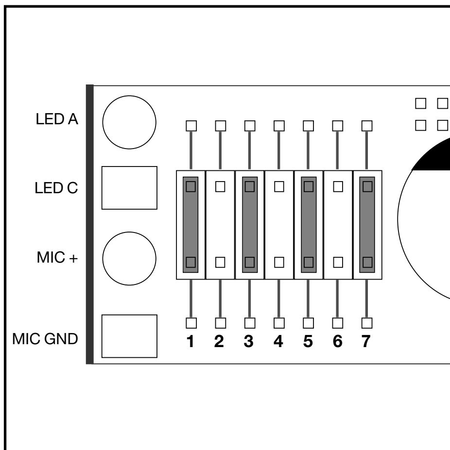
Fig. 2: DPA-P jumpers and pinout (factory setting shown).
