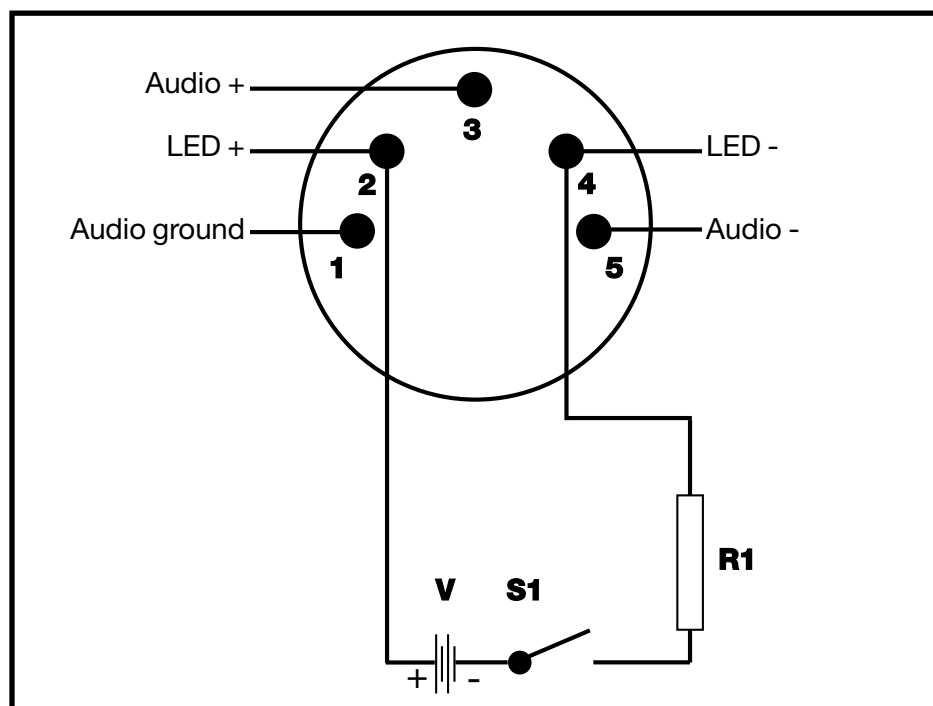
Fig. 5: LED ring external powering.
