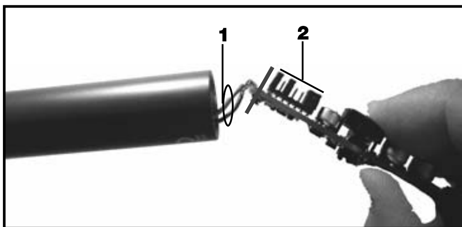
Fig. 3: Inserting the circuit board into the barrel.
