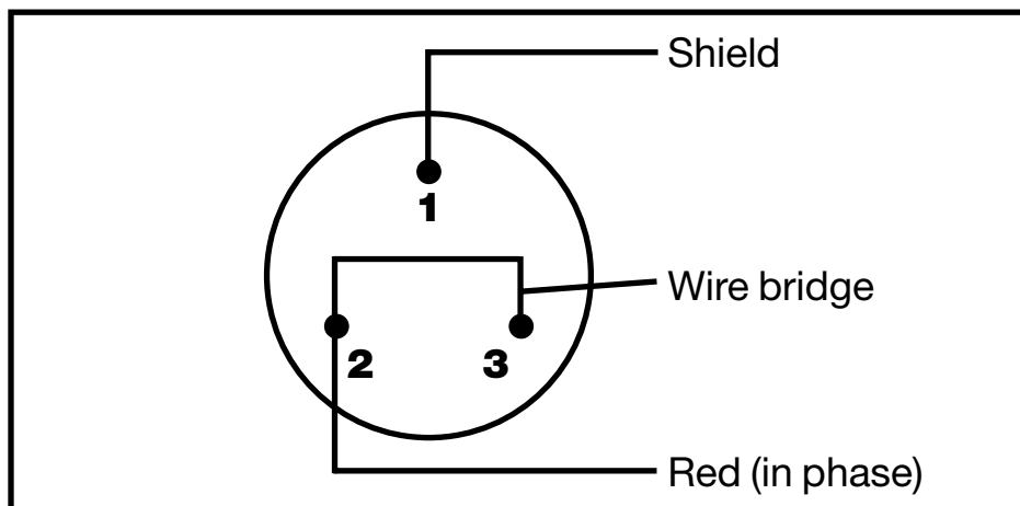
Fig. 6: Connector pinout for connecting to bodypacks
