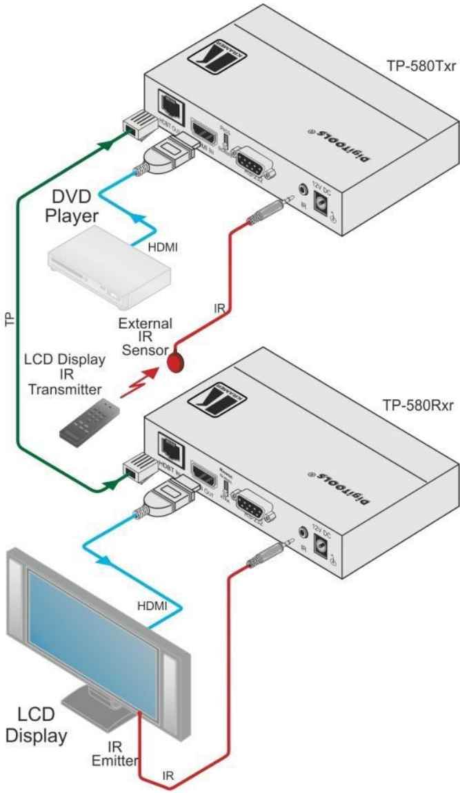
Figure 5: Controlling an LCD Display via the TP-580Txr
