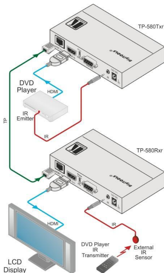
Figure 4: Controlling a DVD Player via the TP-580Rxr
