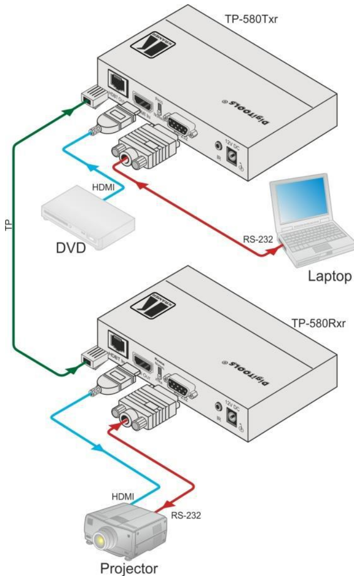
Figure 6: RS-232 Control
