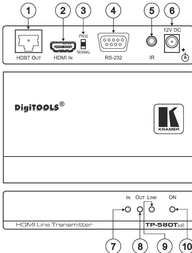
Figure 1: TP-580Txr HDMI Line Transmitter
