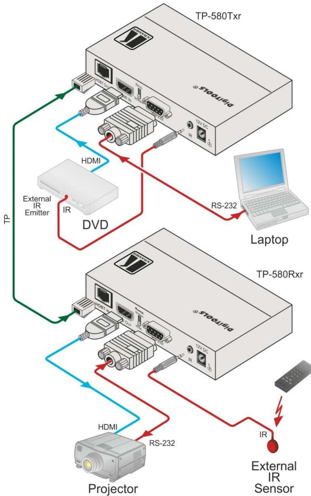
Figure 3: Connecting the TP-580Txr/TP-580Rxr Transmitter/Receiver
