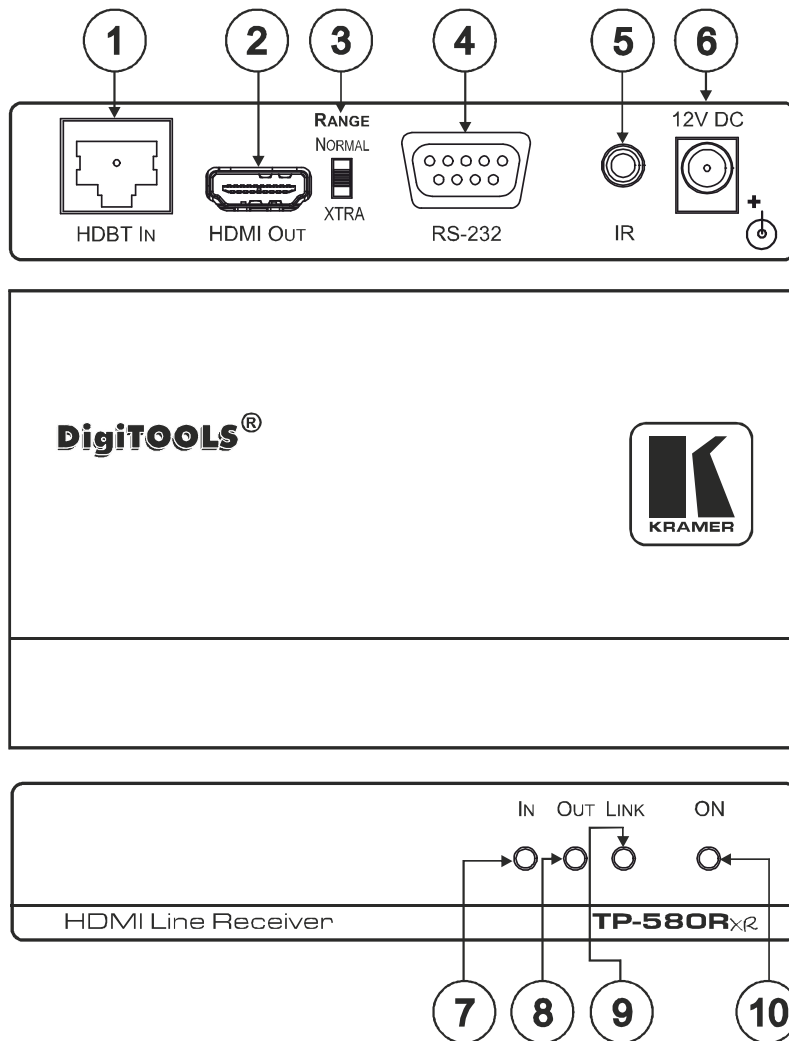
Figure 2: TP-580Rxr HDMI Line Receiver
