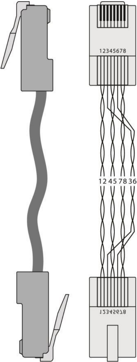
Figure 7: TP PINOUT
